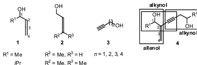
Figure 1. Structures of allenol, alkynol, and allenyne 1,6-diol.
