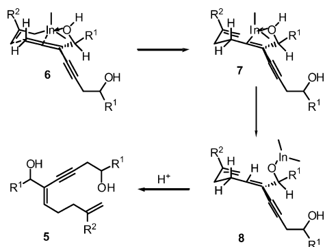
Scheme 1. Plausible mechanism for the addition of allylindiums to allenyne 1,6-diol.
